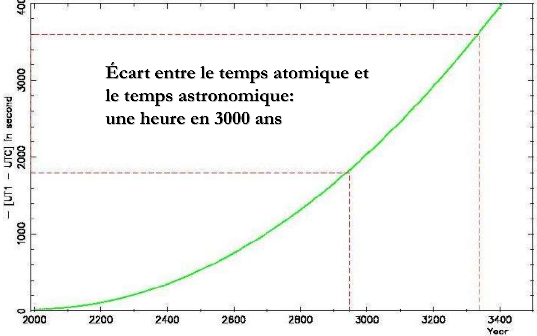
Quadratic Evolution of - [UT1 - TA] wrt Years with the mean Dlod = 2 ms
